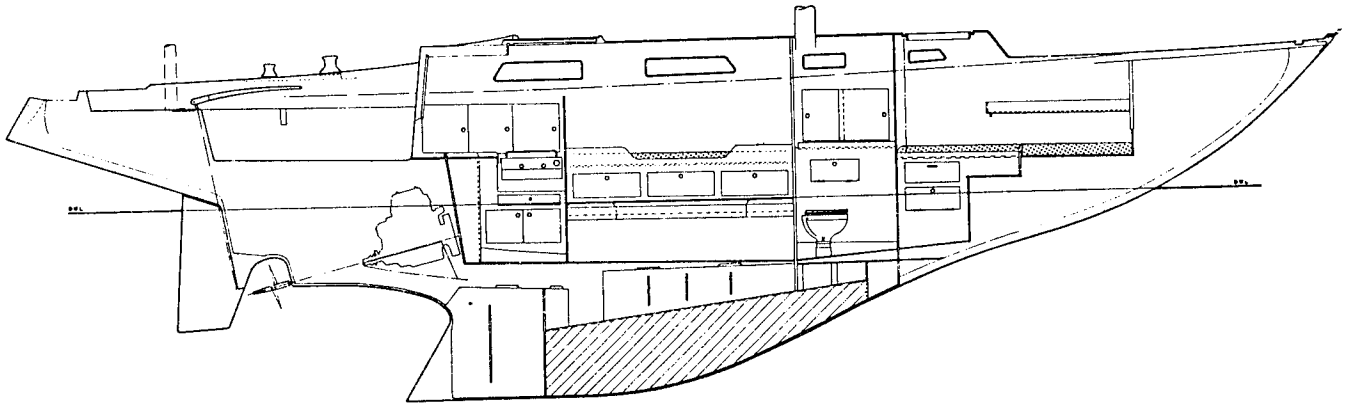
SECTION LOOKING TO PORT
