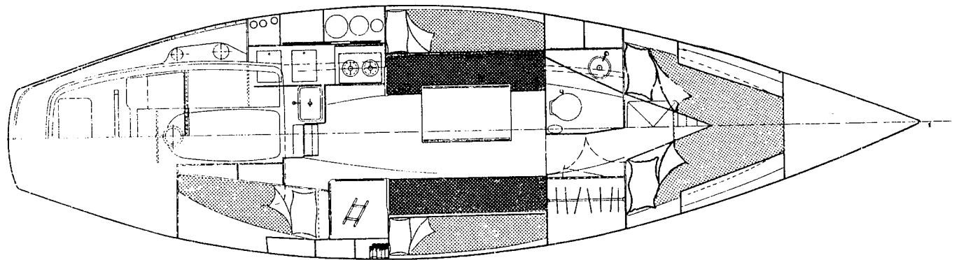
PLAN LAYOUT
